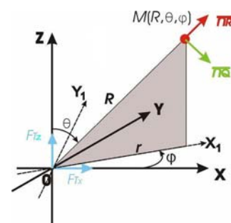
Fig. 1. Calculation scheme for field of normal F_z or tangential F_x harmonic force source
