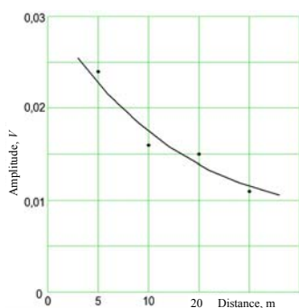
Fig. 13 Echo-signal amplitude from the rail's butt-end versus the distance between the antenna array and the butt-end
