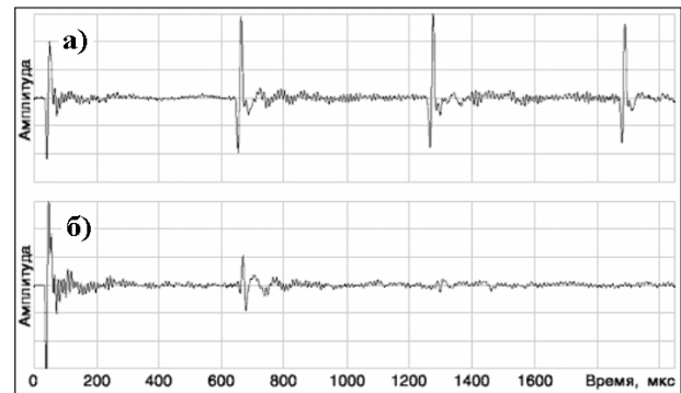
Fig. 12. Echo-signal oscillograms received on anchor bolt end: (a) free lying bolt; (b) built-in concrete bolt
