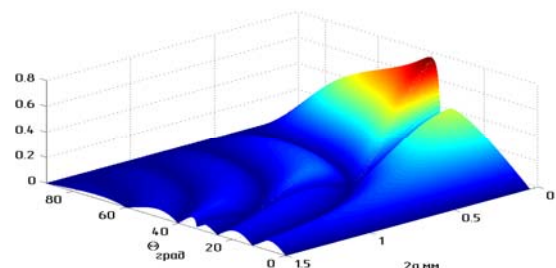
Fig. 6. Dependence of shear wave normal value module as a function of two variables - width of the element 2a and angle \theta at \varphi = 0
