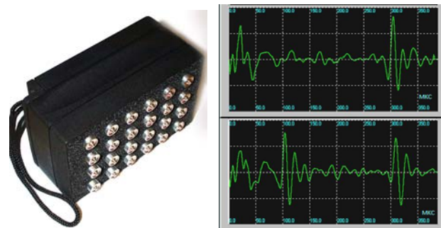
Fig. 9. 24-element antenna array built from SATs with DPC for concrete thickness measurement and received echo-signals
