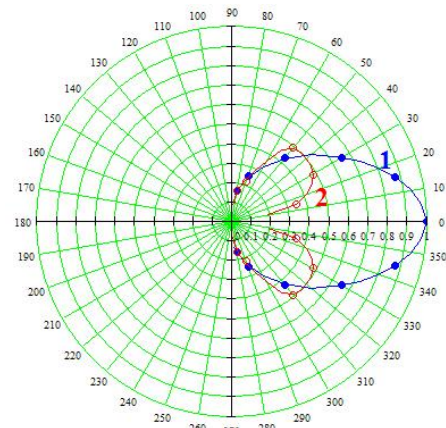
Fig. 17. Directivity pattern of longitudinal and shear waves for a single high-frequency SAT of antenna array with a liquid contact
