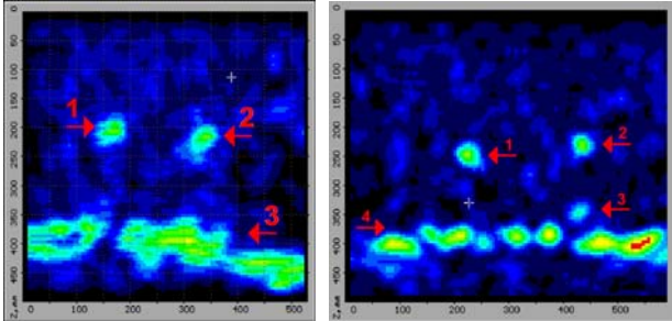
Fig. 10. Tomograms of a concrete block with internal artificial defects, obtained after testing with 36 element antenna array
