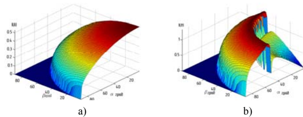
Fig. 2. 3D directivity pattern for SAT with DPC with a normal vibration of wear tip: a – for longitudinal wave; b – for shear wave
