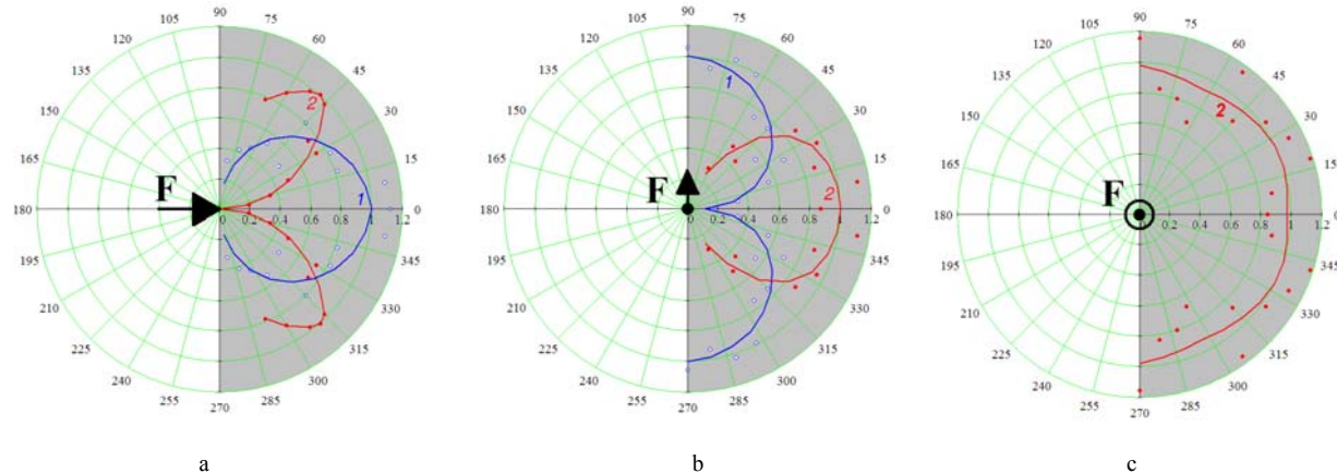
Fig. 8. Directivity patterns of transducers with DPC: a – with normal vibration of the wear tip; b – with tangential vibration of the type, section along the vibration vector; c – with tangential vibration of the type, section perpendicular to oscillation vector; 1 – longitudinal waves; 2 – shear waves
