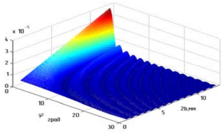
Fig. 7. Dependence of shear oscillations as a function of parameters 2b and \varphi at \theta = 50^\circ
