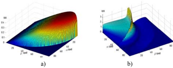
Fig. 3. 3D directivity pattern for SAT with DPC with a tangential vibration of wear tip: a – for longitudinal wave; b – for shear wave
