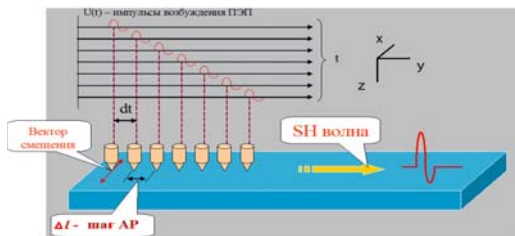
Fig. 4. SH-wave for guided wave testing
